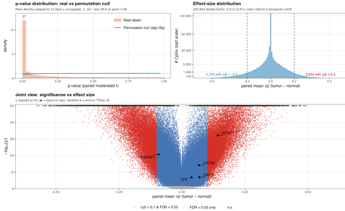
Figure 2: Paired tumor-normal DM diagnostic. Top-left: p-value distribution — real labels (peach; leftmost bin density 27, capped at 12 for plotting) vs sign-flip permutation null (blue, flat at \approx 1 ); \lambda_{GC}^{\text{real}} = 36.8 vs \lambda_{GC}^{\text{perm}} = 0.95 visualizes that the inflation is real signal, not miscalibration. Top-right: paired-mean \Delta\beta on a sqrt scale; 9,312 CpGs (2.9%) clear |\Delta\beta| > 0.2 . Bottom: volcano on paired mean \Delta\beta (y capped at 50; triangles = beyond cap) with five anchor TSGs — SFRP1/GATA5/DKK3 hypermethylated, VHL near origin (subgroup-driven, cohort-mean \Delta\beta \approx 0 ), RASSF1 hypomethylated (§4.2).
